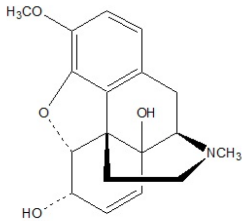
14-Hydroxycodeine
